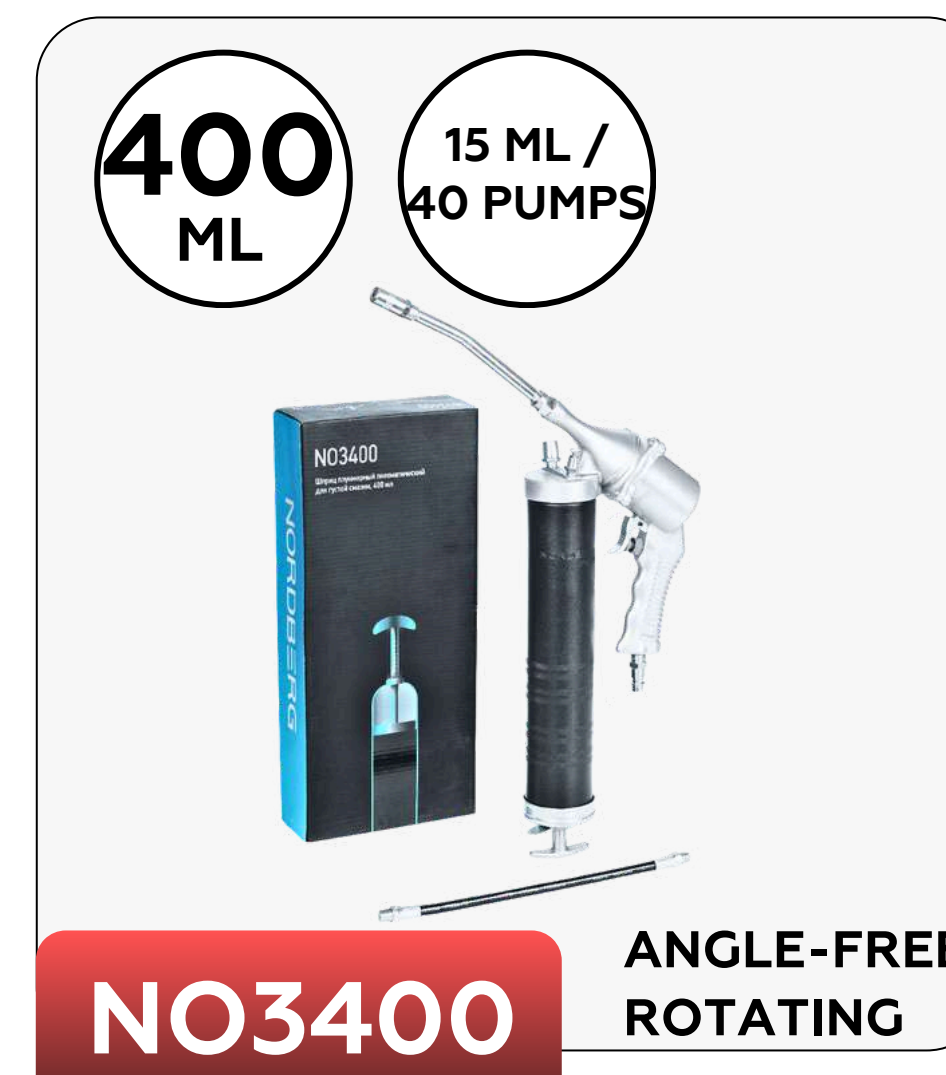
NO3400 ANGLE-FREE ROTATING CONTINUOUS FLOW AIR GREASE GUN 400 ML 110 AED
